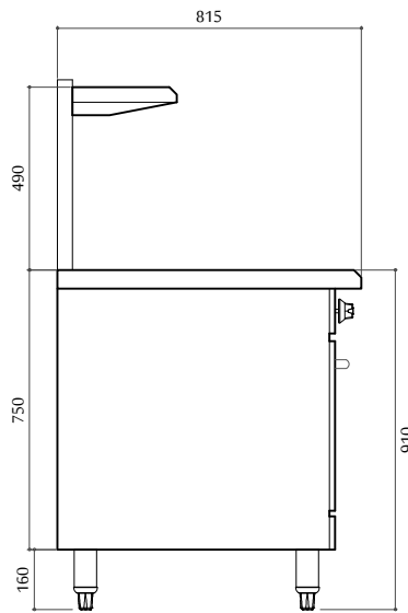
SIDE ELEVATION
