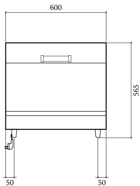
FRONT ELEVATION
